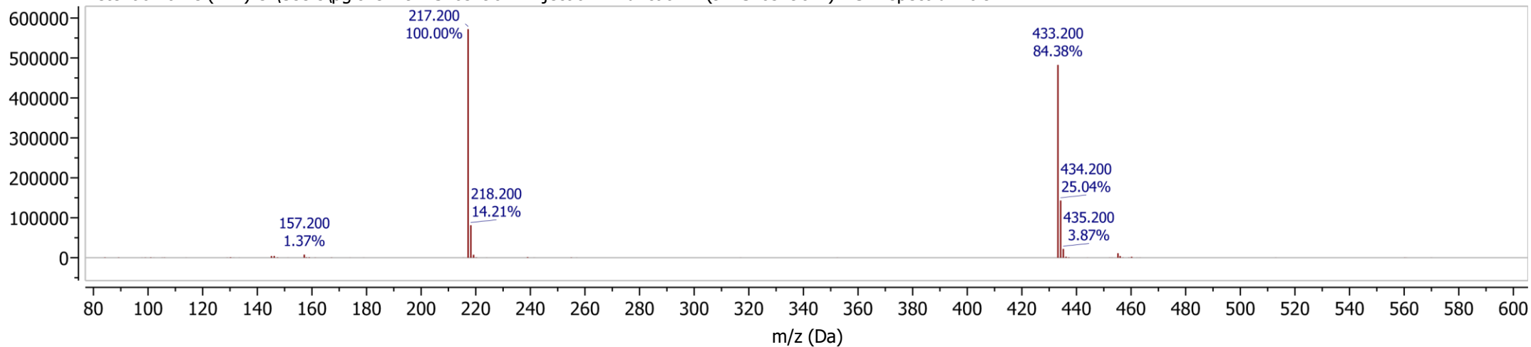
Retention time (min) C:\Users\pglche... 9-RS283298.D Injection 1 Function 1 (9-RS283298.D) MS + spectrum 0.97
