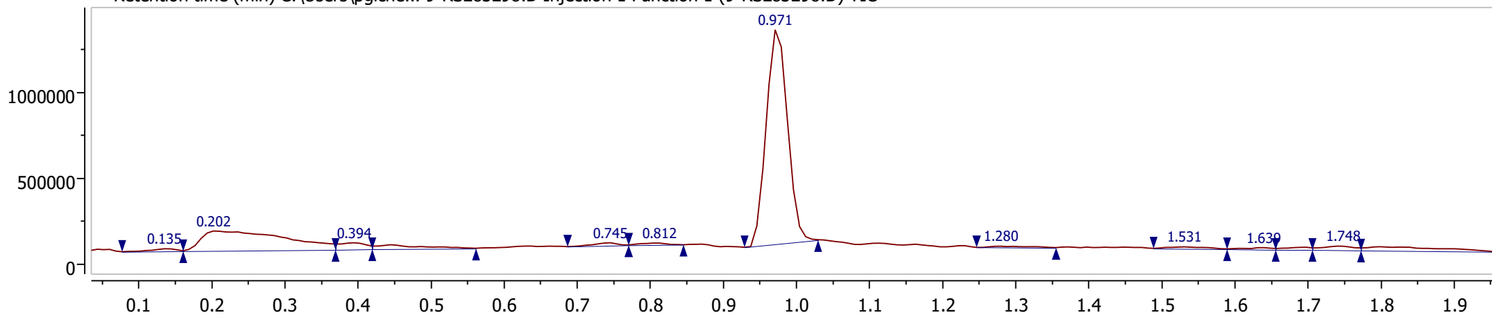
Retention time (min) C:\Users\pglche... 9-RS283298.D Injection 1 Function 1 (9-RS283298.D) MS + spectrum 0.97
