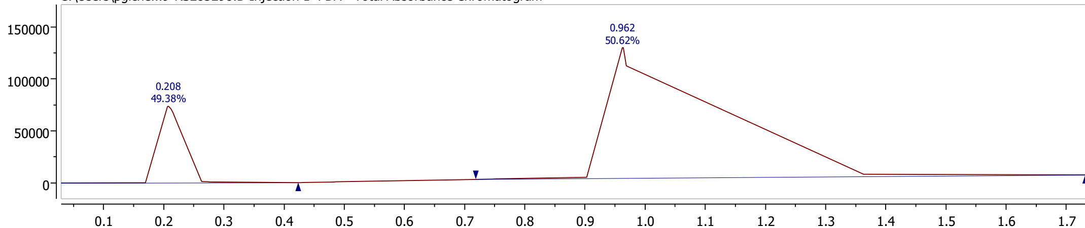
Retention time (min) C:\Users\pglche... 9-RS283298.D Injection 1 Function 1 (9-RS283298.D) TIC
