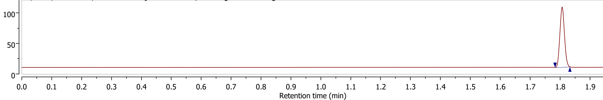
C:\Users\retro...5chA\CAD031LCMS Injection 1 Function 2 MS - spectrum 0.05
