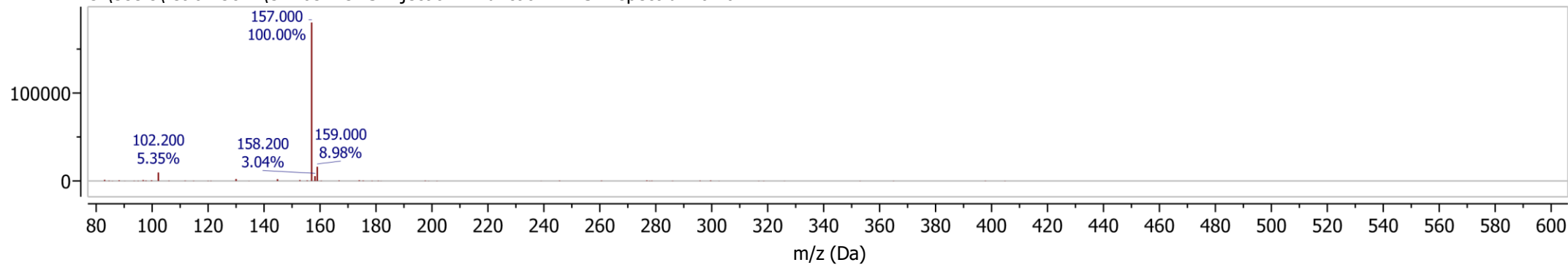
C:\Users\retro...5chA\CAD031LCMS Injection 1 ELS1A, ELSD Signal Chromatogram
