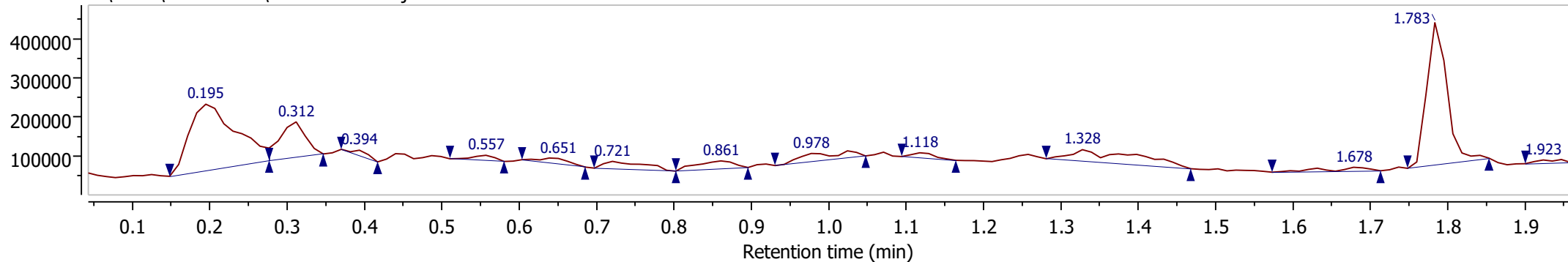
C:\Users\retro...5chA\CAD031LCMS Injection 1 Function 1 MS + spectrum 0.20
