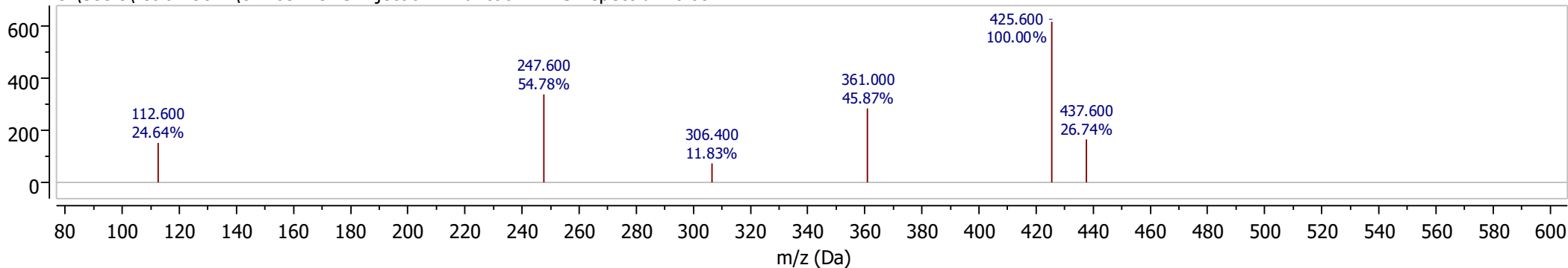
C:\Users\retro...5chA\CAD031LCMS Injection 1 Function 2 MS - spectrum 0.05
