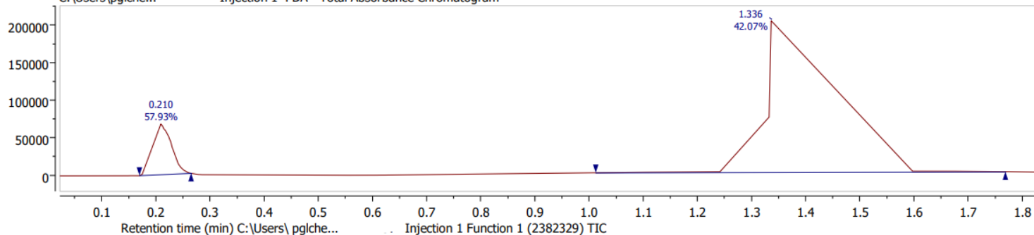
C:\Users\pglche... Injection 1 PDA - Total Absorbance Chromatogram
